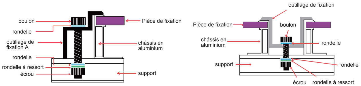
Figure 5 Clamp installation guideline
